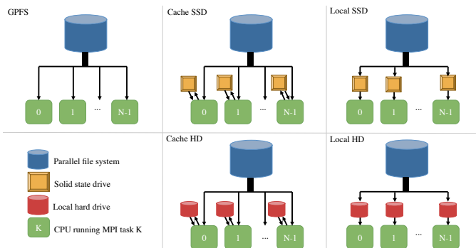
Fig. 5: Test configurations.
