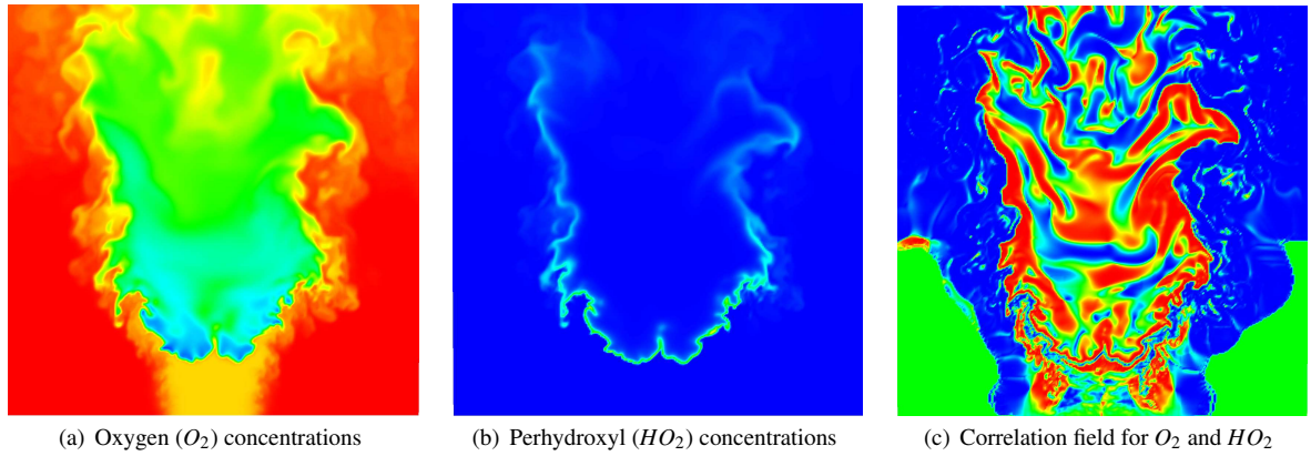
(a) Oxygen ( O_2 ) concentrations (b) Perhydroxyl ( HO_2 ) concentrations (c) Correlation field for O_2 and HO_2
