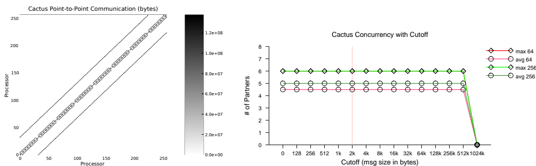
Figure 6: Cactus (a) volume of communication at P=256 and (b) effect of thresholding on TDC for P=64,256
