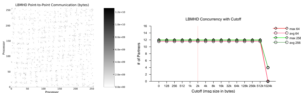
Figure 7: LBMHD (a) volume of communication P=256 and (b) effect of thresholding on TDC for P=64,256
