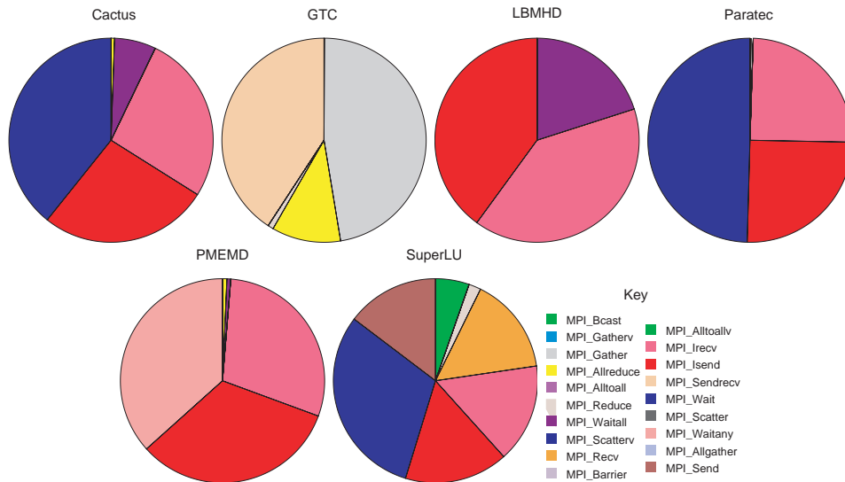
Figure 2: Relative number of MPI communication calls for each of the codes.
