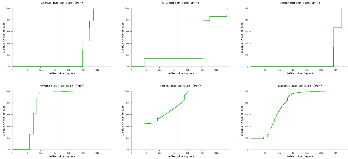
Figure 4: Buffer sizes distribution for point-to-point communication. The pink line demarcates the bandwidth-delay product.
