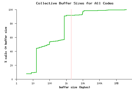
Figure 3: Buffer sizes distribution for collective communication for all codes. The pink line demarcates the bandwidth-delay product.
