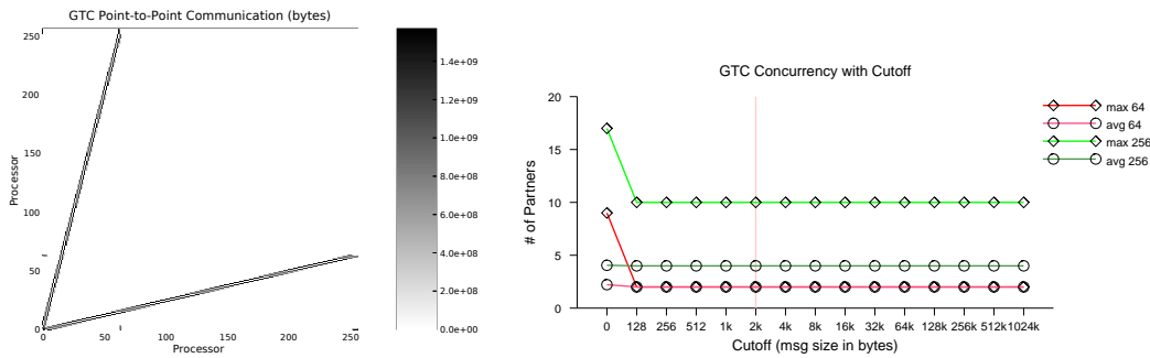
Figure 5: GTC (a) volume of communication at P=256 and (b) effect of thresholding on TDC for P=64,256
