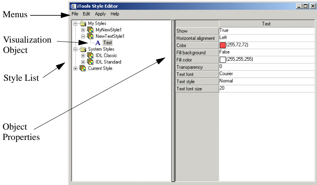
Figure 9-9: The iTools Style Editor
