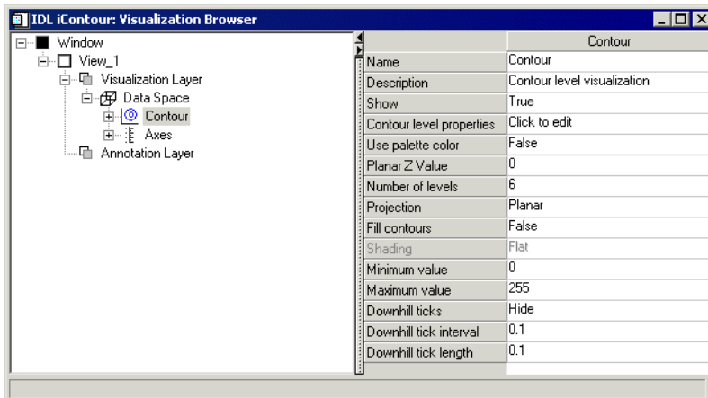
Figure D-15: Visualization Browser with Contour Properties Displayed
