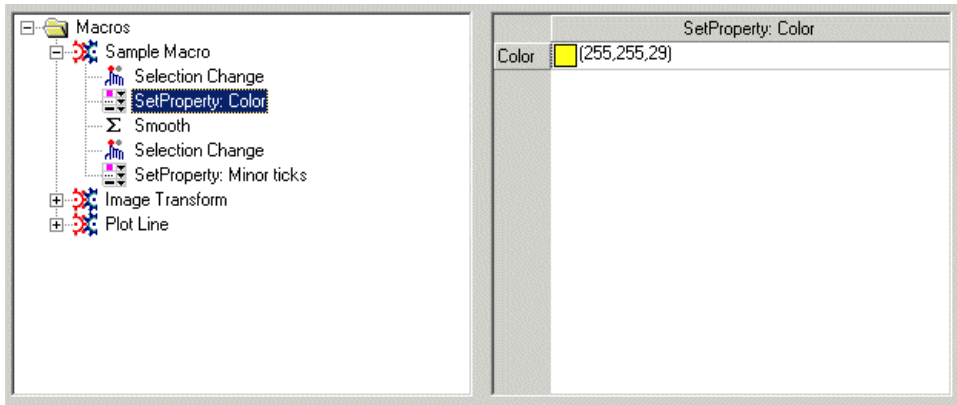
Figure 8-15: Macro Items in the Macro Editor
