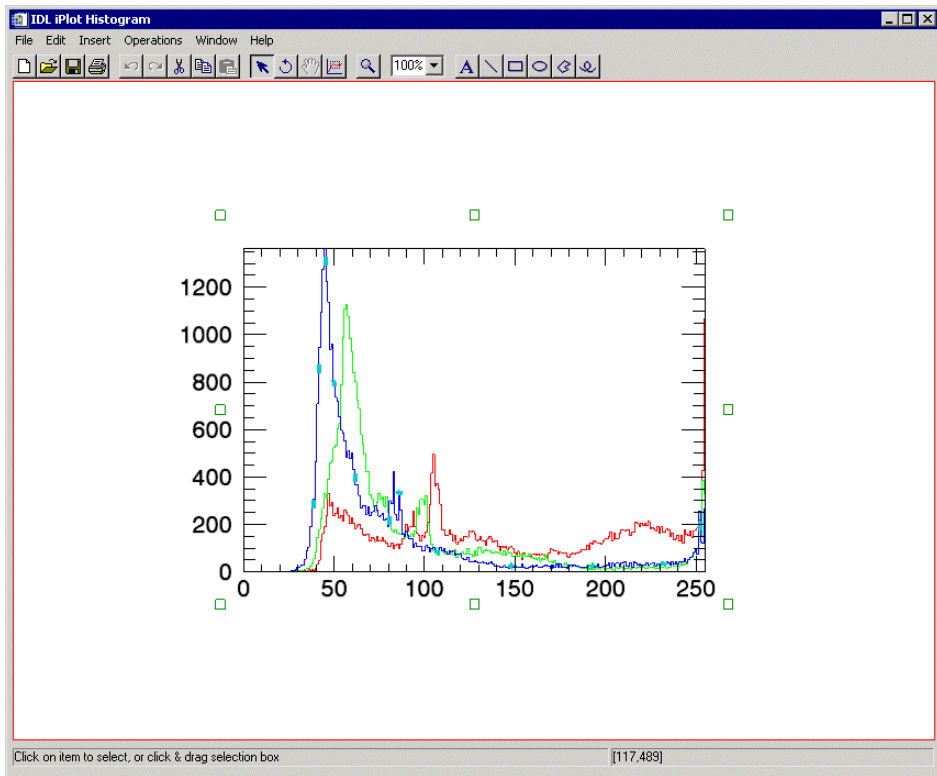
Figure 7-11: Histogram Plot
