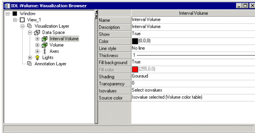
Figure D-20: Visualization Browser with Interval Volume Properties Displayed
