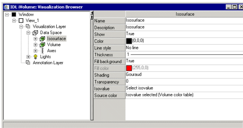
Figure D-19: Visualization Browser with Isosurface Properties Displayed
