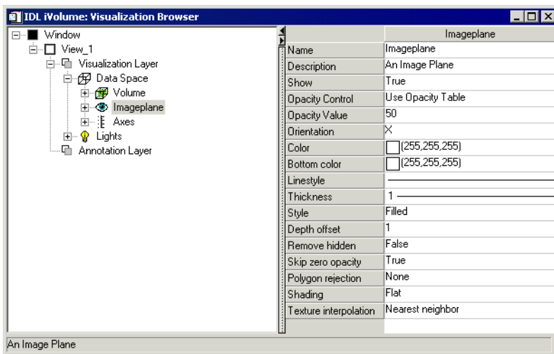
Figure D-21: Visualization Browser with Image Plane Properties Displayed
