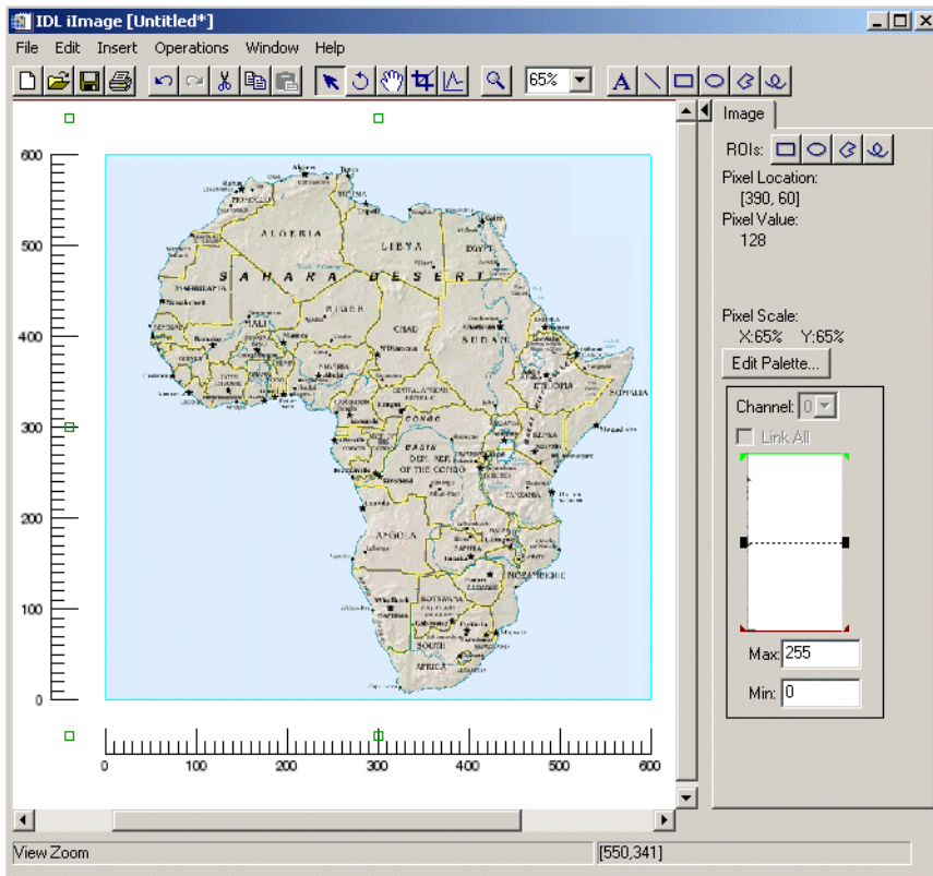
Figure 10-6: Image in ilimage with Axes Inserted and Placed
