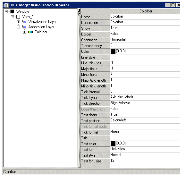
Figure D-30: Visualization Browser with Colorbar Properties Displayed
