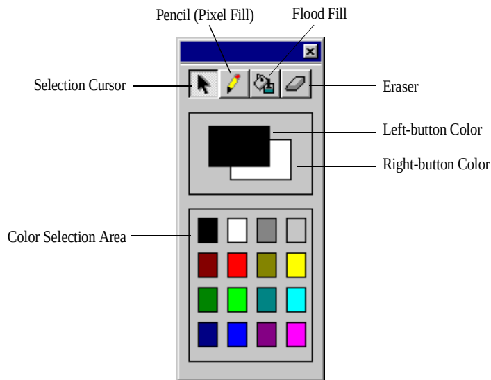
Figure 23-10: Bitmap Editor Tools
