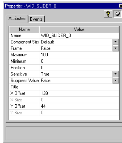
Figure 23-7: Properties Dialog for a Slider Widget
