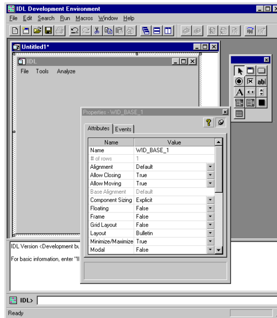
Figure 23-3: IDL GUIBuilder with Example Application
