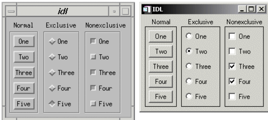
Figure 26-2: Normal Menus (left), Exclusive Menus (center) and Non-exclusive Menus (right)
