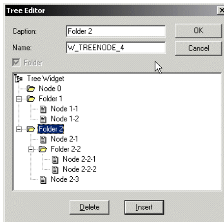
Figure 23-11: Tree Editor Dialog
