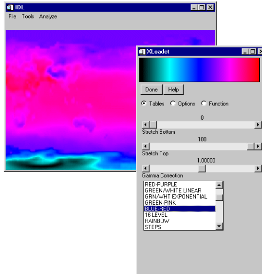
Figure 23-5: Running Example Application and XLOADCT Dialog
