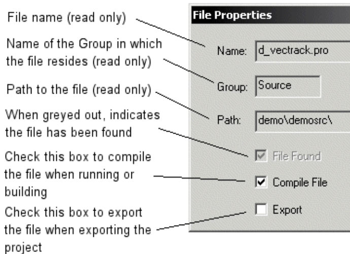
Figure 13-7: File Properties Dialog
