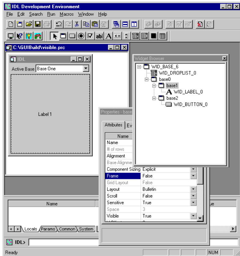
Figure 23-13: Visible Widgets Example Application
