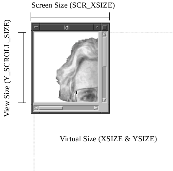
Figure 26-7: Visual description of widget sizes.
